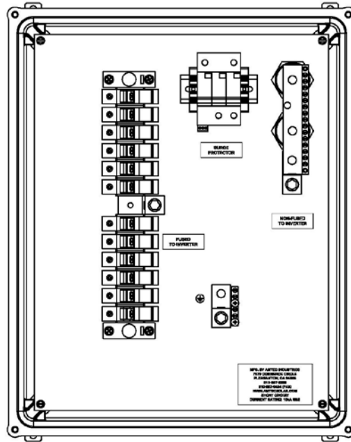
FRONT VIEW – INTERNAL
