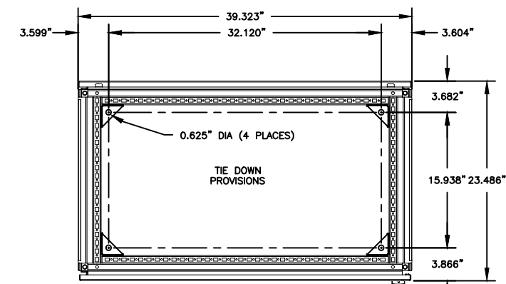
SECTION A - A FRONT
